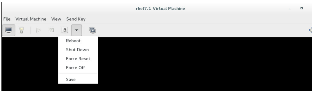
Figure 48 Graceful Shutdown
