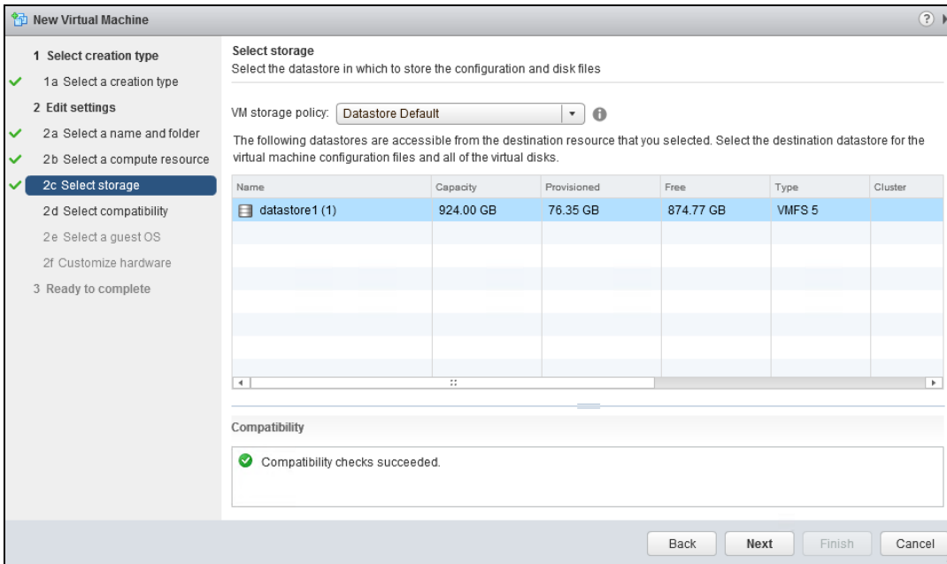
Figure 32 Select Datastore
