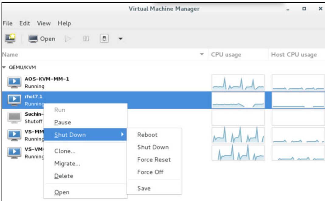
Figure 62 Graceful Shutdown
