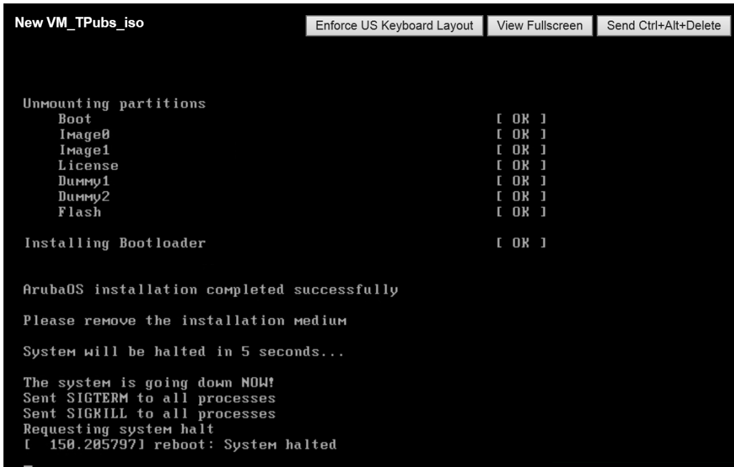
Figure 39 System Halt
