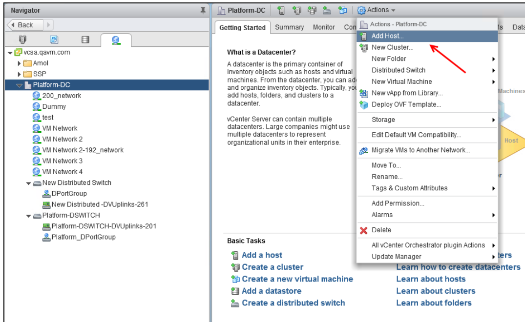
Figure 70 Add Hosts
