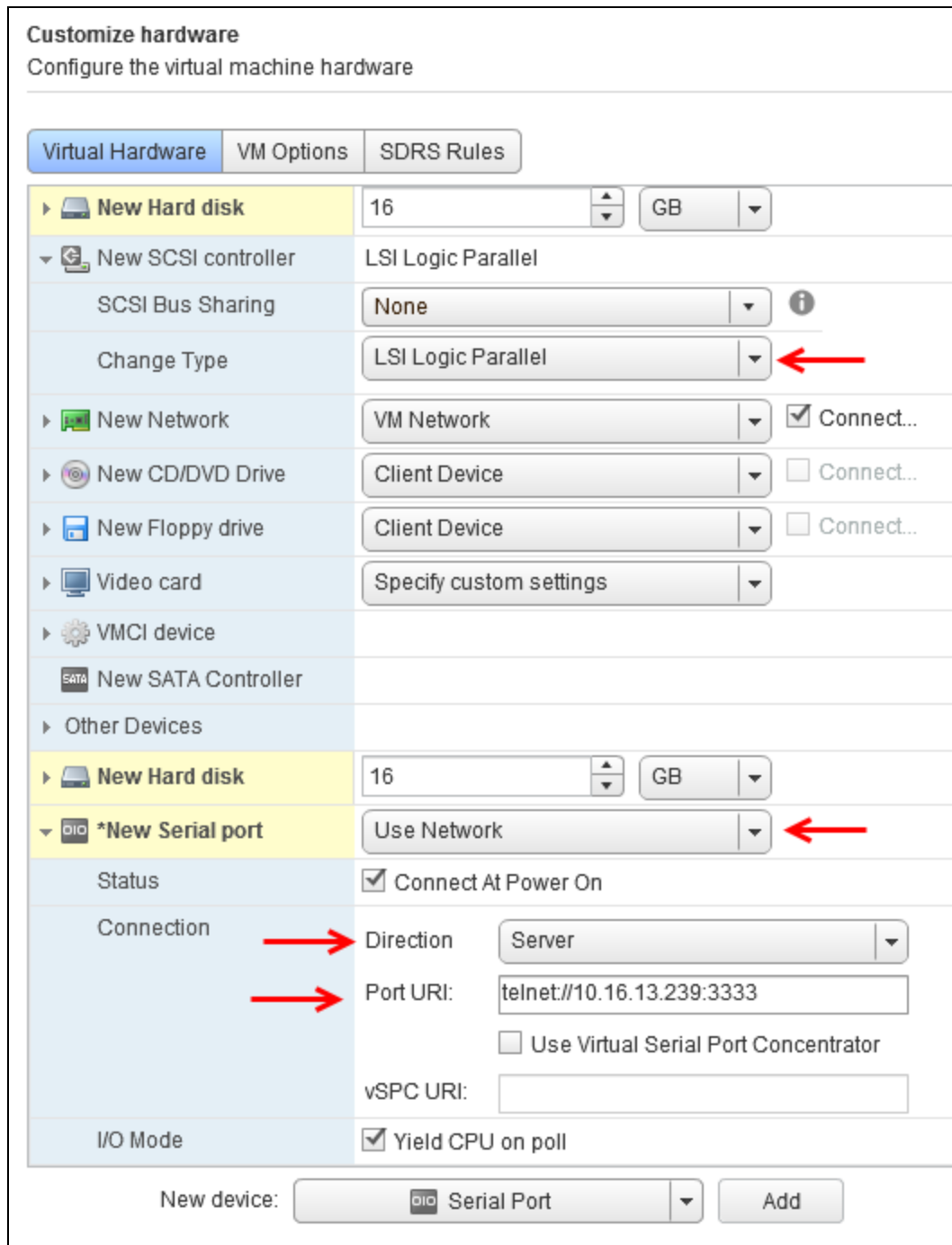
Figure 35 Other Modifications
