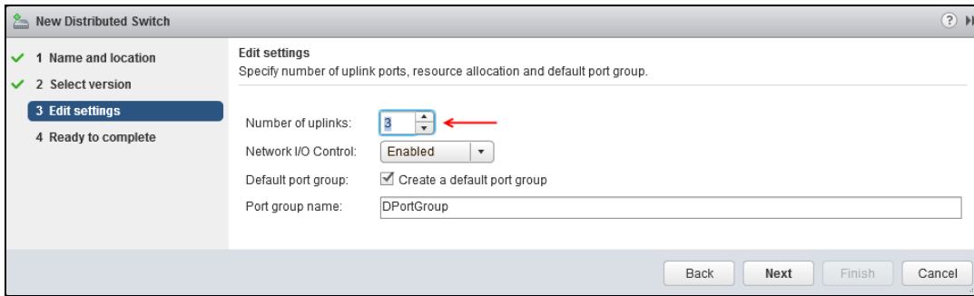
Figure 67 Edit Settings
